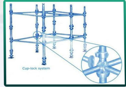
Cuplock system
