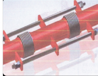
Universal Tied Expansion Joints
