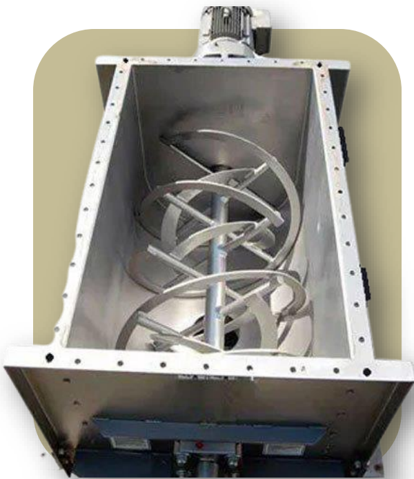
RIBBON BLENDER
