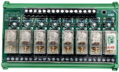
8 Channel Relay Card
