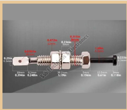
12V Car Bonnet Alarm Light Hood Door Pin Switch
