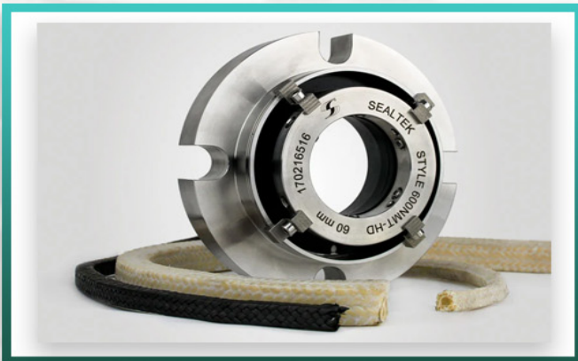
Mechanical Seals and Gland Packing
