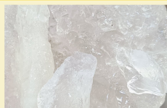
Aluminum Ammonium Sulfate
