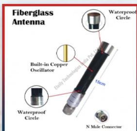
ET-86510FG4-2L3-SMS 865MHz 10dBi Fiberglass Antenna
