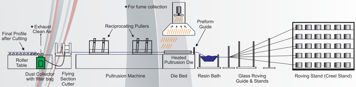
Basic Pultrusion Machine Layout
