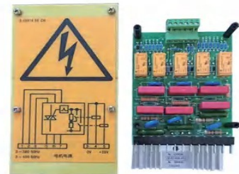
VAC Slewing Block M-61406-43
