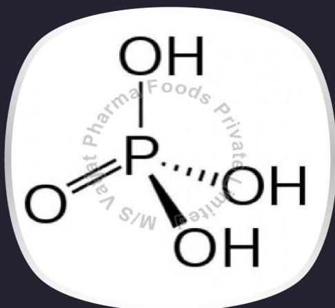
Orthophosphoric Acid
