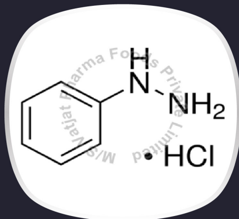
Phenylhydrazine hydrochloride
