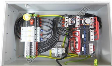
STAR DELTA STARTER CONTROL PANEL
