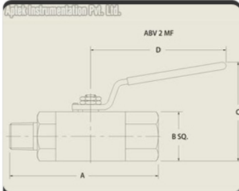
ABV 2 MF High Pressure Ball Valve
