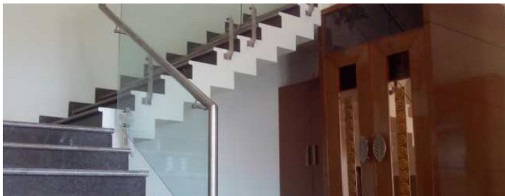
Material : Stainless Steel 304 / 316 | Finish : Matt / Glossy Function : Connects Glass & Handrails Installation : Side Mounted railing with glass and fittings
