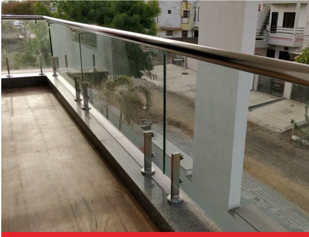
50x10mm Short Height Baluster with glass and fittings 20x40mm Short Height Baluster with glass and fittings 40x40mm Short Height Baluster with glass and fittings
