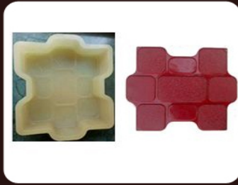
CP - 30 Gem Stone Rubberised PVC Interlocking Paver Moulds
