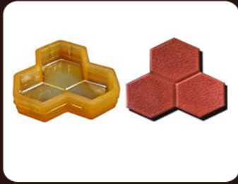
CP - 15 Trihex Rubberised PVC Interlocking Paver Moulds
