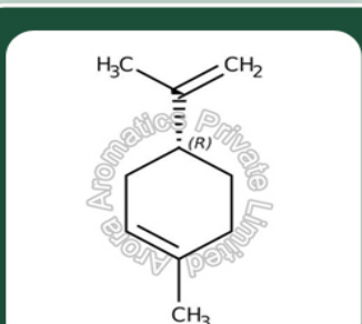
D-Limonene
