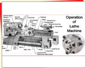
Lathe Machine
