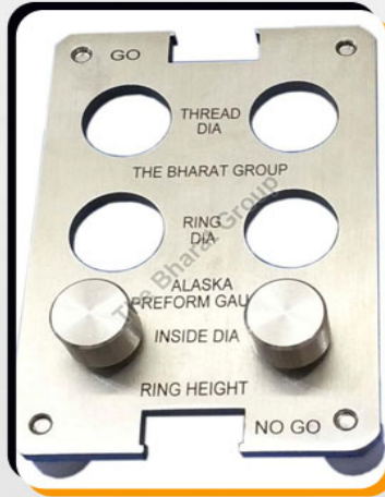
Preform Go No Go Gauge
