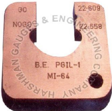
Fixed Type Snap Gauge
