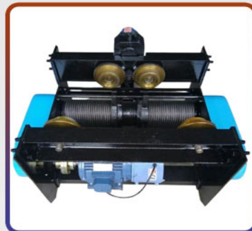
Electrical Wire Rope Hoist
