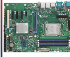
Advantech AIMB-723 ATX Motherboard
