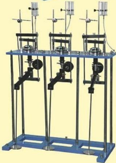
Consolidation Test Apparatus
