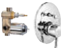
High flow single lever concealed diverter system consisting of Exposed part (lever, tip ton knob, wall flange) and Concealed part (45 mm cartridge with button assembly, cartridge sleeve)
