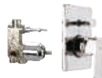
5-way single lever concealed diverter system consisting of Exposed part (lever, tip ton knob, flange) and Concealed part (cartridge with button assembly, cartridge sleeve) Exposed part F1005711 ₹ 2375 Concealed part F4020101 ₹ 3645 Set ₹ 6020
