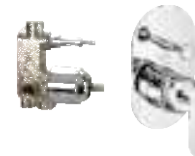
5-way single lever concealed diverter system consisting of Exposed part (lever, tip ton knob, flange) and Concealed part (cartridge with button assembly, cartridge sleeve) Exposed part F1018711 ₹ 2200 Concealed Part F4020101 ₹ 3645 Set ₹ 5845
