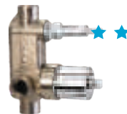
F4010105 Concealed body for turn type single lever concealed diverter system consisting of 35 mm cartridge with button Assembly, Cartridge Sleeve (but without operating lever, wall flange and tip ton knob) Water saving 38%
