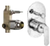
Single lever concealed diverter system consisting of Exposed part (lever, tip ton knob, flange) and Concealed part (35 mm cartridge with button assembly, cartridge sleeve) Exposed part F1018701 ₹ 2100 Concealed Part F4010101 ₹ 2955 Set ₹ 5055
