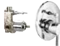
5-way single lever concealed diverter system consisting of Exposed part (lever, tip ton knob, wall flange) and Concealed part (cartridge with button assembly, cartridge sleeve)
