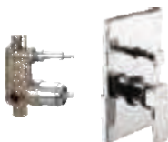
Single lever concealed diverter system consisting of Exposed part (lever, tip ton knob, flange) and Concealed part (35 mm cartridge with button assembly, cartridge sleeve) Exposed part F1005701 ₹ 1825 Concealed part F4010103 ₹ 2710 Set ₹ 4535
