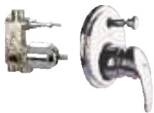
5-way single lever concealed diverter system consisting of Exposed part (lever, tip ton knob, flange) and Concealed part (cartridge with button assembly, cartridge sleeve) Exposed part F1001711 ₹ 1940 Concealed part F4020101 ₹ 3645 Set ₹ 5585
