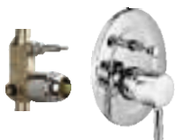
Single lever concealed diverter system consisting of Exposed part (lever, tip ton knob, wall flange) and Concealed part (40 mm cartridge with button assembly, cartridge sleeve)
