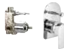
5-way single lever concealed diverter system consisting of Exposed part (lever, tip ton knob, flange) and Concealed part (cartridge with button assembly, cartridge sleeve)
