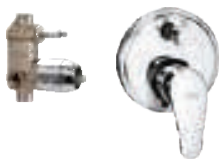
Turn type single lever concealed diverter system consisting of Exposed part (lever, turn type knob, flange) and Concealed part (35 mm cartridge with button assembly, cartridge sleeve) Exposed part F1001703 ₹ 1415 Concealed part F4010105 ₹ 3250 Set ₹ 4665
