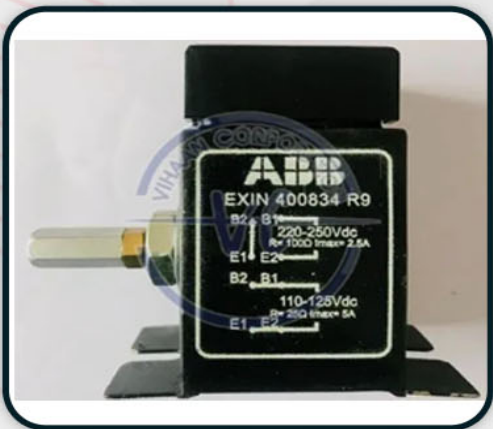
ABB Tripping Coil
