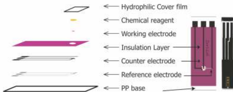
Screen-Printed Carbon Electrode
