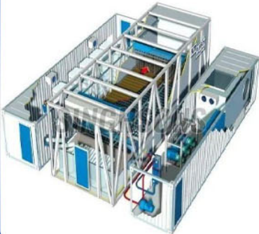
Automatic Block Ice Plant
