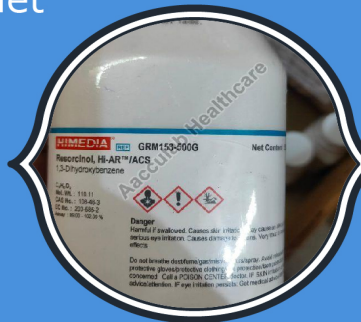
Resorcinol
