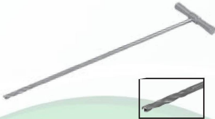
Cannulated Rigid Reamer
